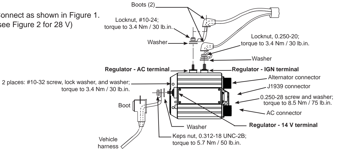
FIGURE 1 – Installing N3223 in 28/14 V Applications
