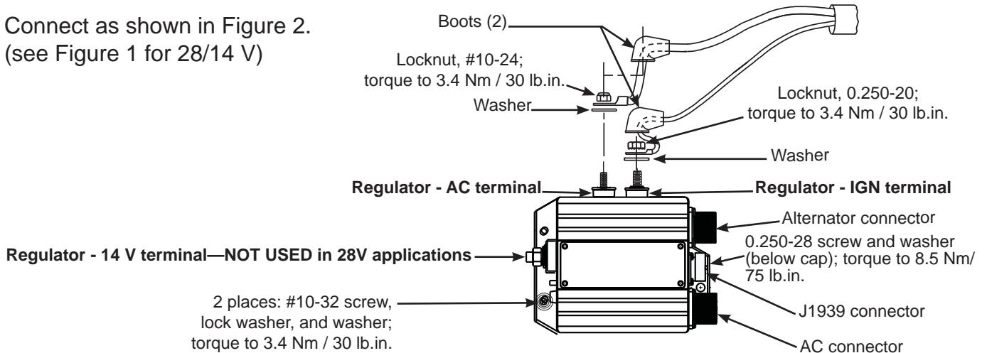
FIGURE 2 – Installing N3223 in 28 V Applications
