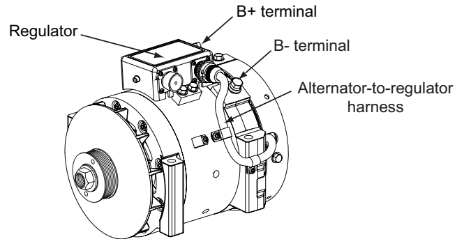
Figure 1: C535 Alternator Terminals
