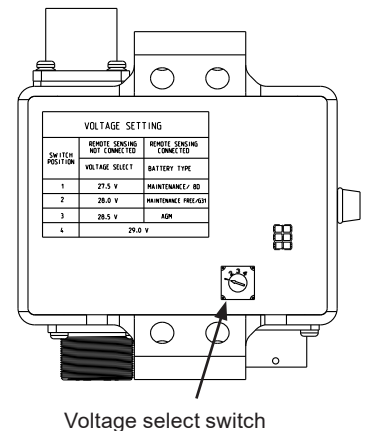
Figure 4: A2-398 Voltage Regulator Features
