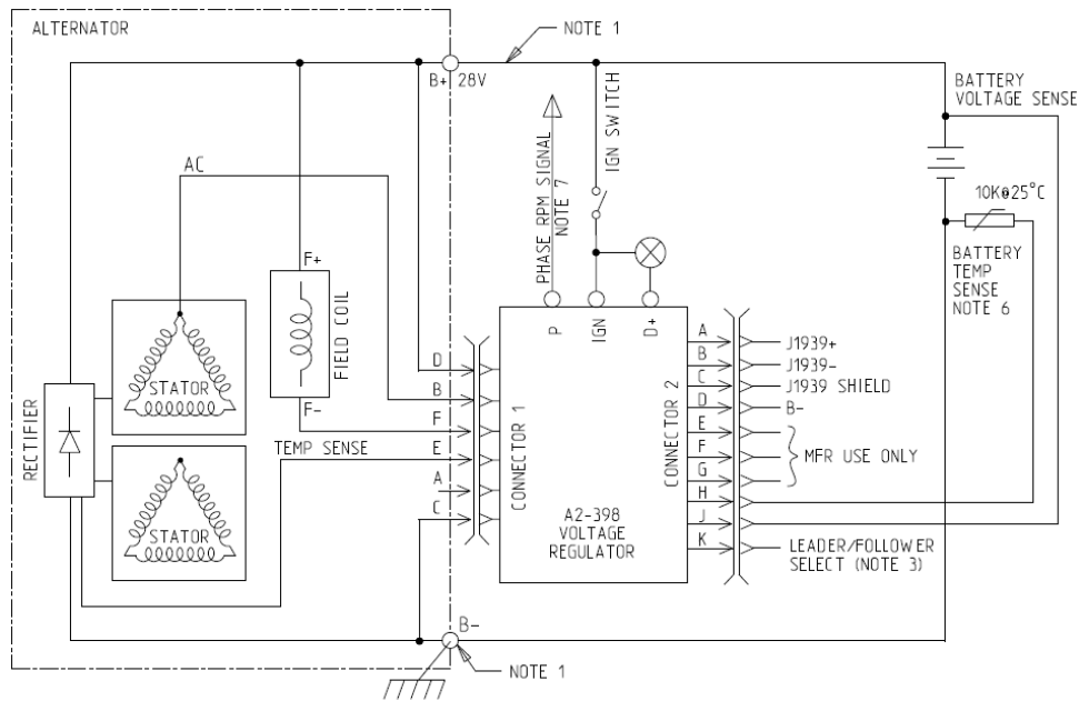
Figure 3: C535 Alternator with Regulator Wiring Diagram
